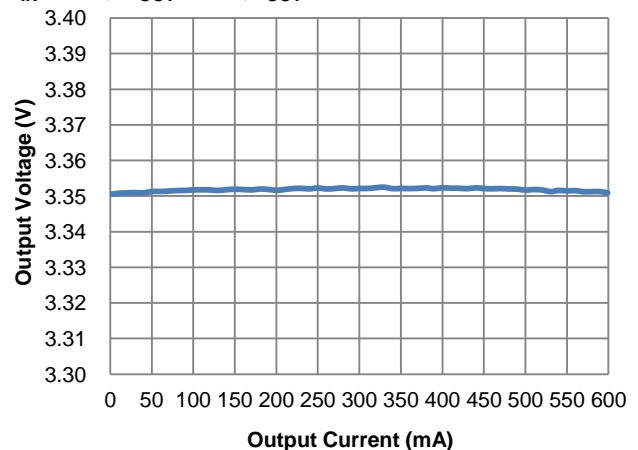
Figure 13. Output Voltage vs. Output Current
