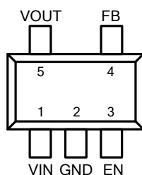
Figure 1. Pin Assignments of FP6186A
